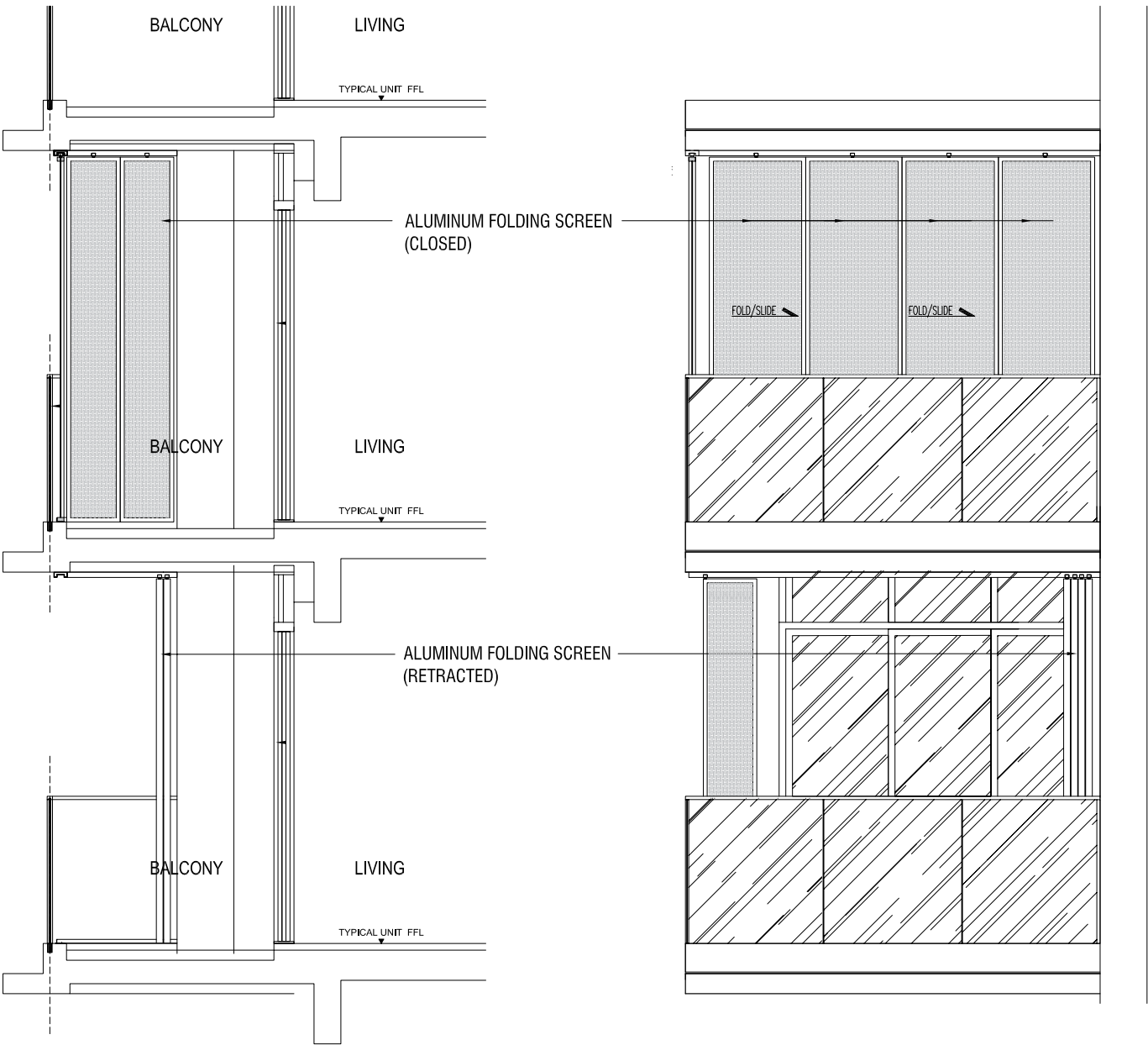
SECTION A-A (TYPICAL SECTION OF BALCONY / PES SCREEN)
